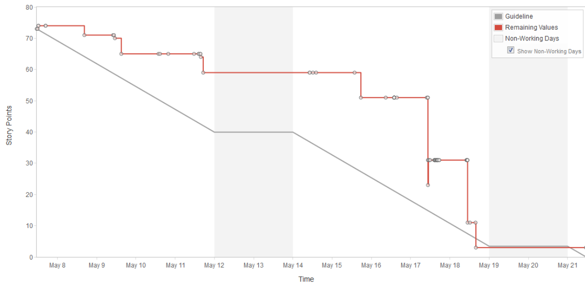
Figure 2 Burndown Chart Sprint 2
