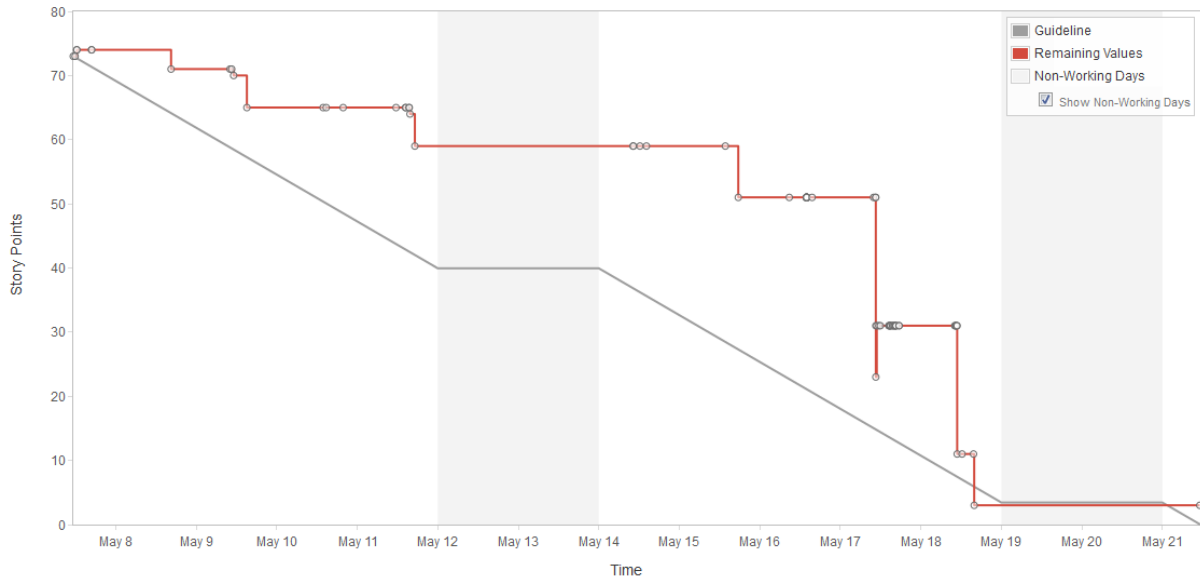
Figure 1 Burndown Chart Sprint 1
